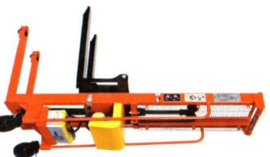
Semi Electric Stacker (LD) CAPACITY 1000 Kgs LIFTING HEIGHT 1600 mm
